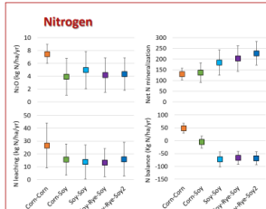
Fig. 2: 30-year average values of N 2 O emissions, net N mineralization, N leaching, and N balance (N applied + N fixation – grain N) per cropping system.
